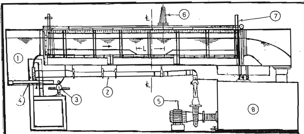
Fig. 1 Schematic sketch of test facility
