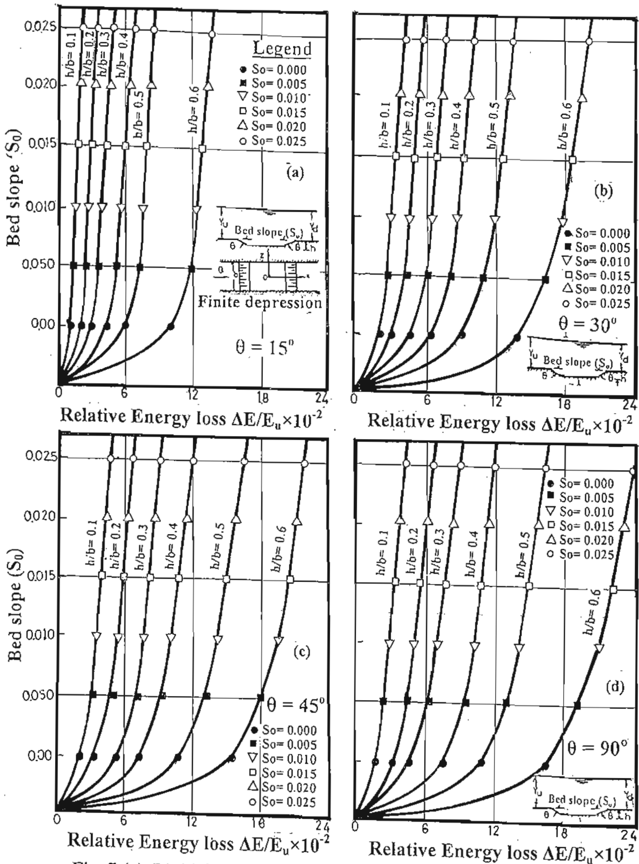
Fig. 7 (a),(b),(c)&(d) Variation of relative energy loss \Delta E/E_u with bed slope S_o for different values of relative height h/b at different values of angle \theta
