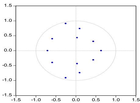
Fig. 2. (VAR) satisfies the stability condition
